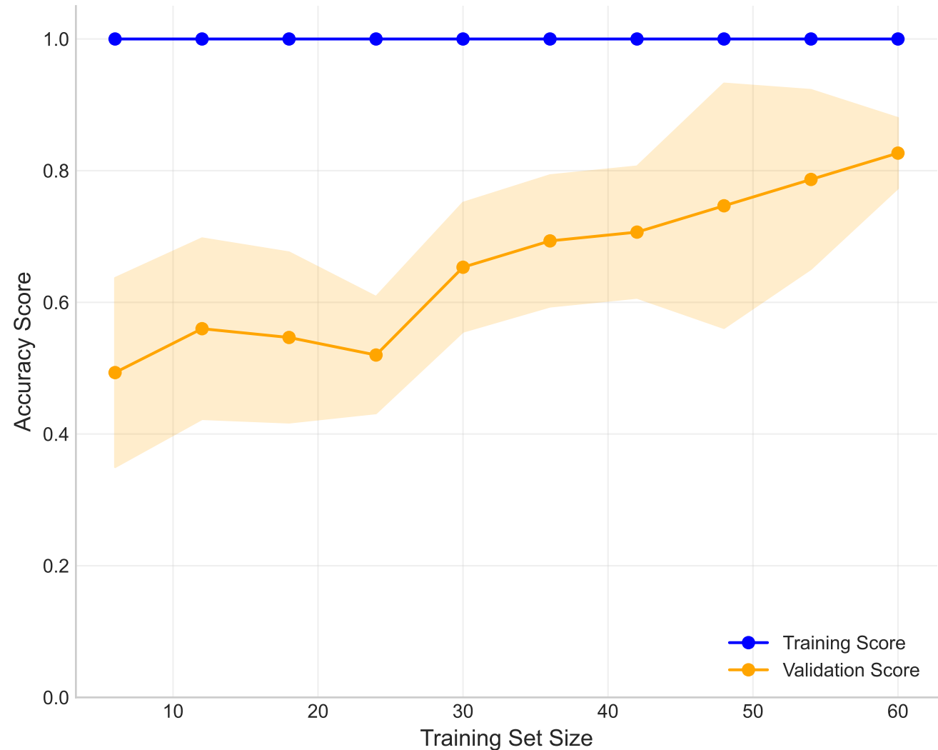
Learning Curves (Avg Gap: 0.347)
