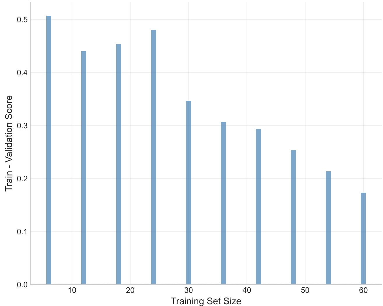
Generalization Gap by Training Size
